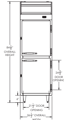
ELEVATION VIEW
