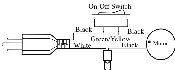
Wiring Diagram (no reset switch)
