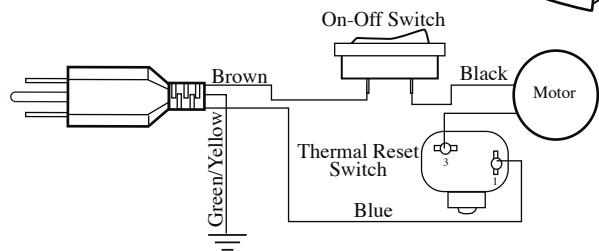
Wiring Diagram (units with reset switch)
