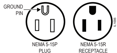
Fig. 3 Plug Configuration
