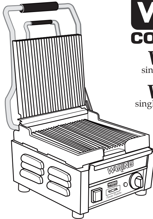
034204 Base Unit Assembly / WPG150T Panini Perfetto
